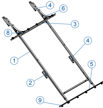
INCLINED SURFACE
