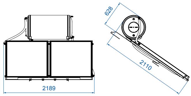
INCLINED SURFACE
