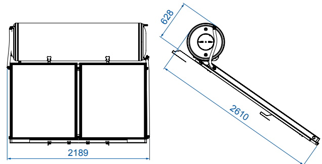
INCLINED SURFACE
