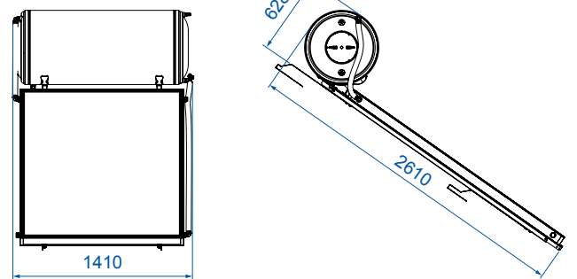
INCLINED SURFACE
