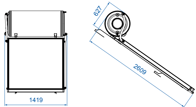
INCLINED SURFACE
